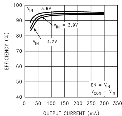
Efficiency vs Output Current ( V_{OUT} = 3.25V )
