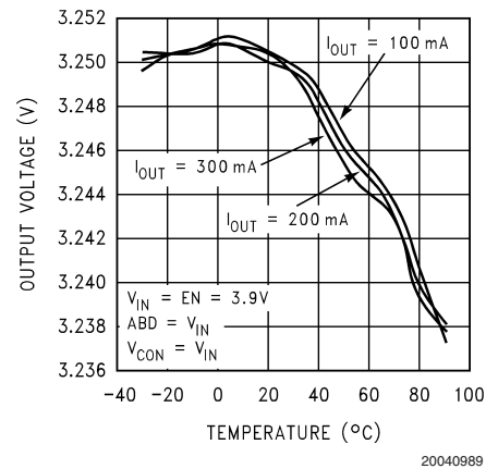
Output Voltage vs Temperature ( V_{OUT} = 3.25V )
